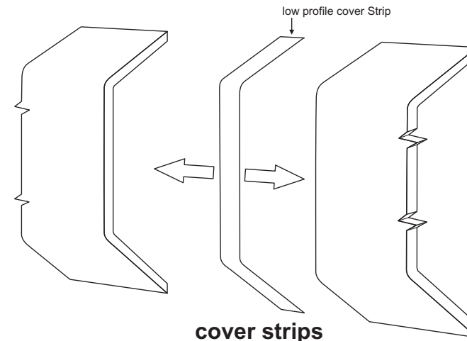
Cover Strip Joint Detail (1 : 2)
